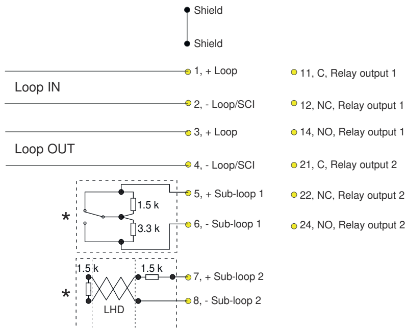
Figure 3. Linear Heat Detection (LHD) cable
