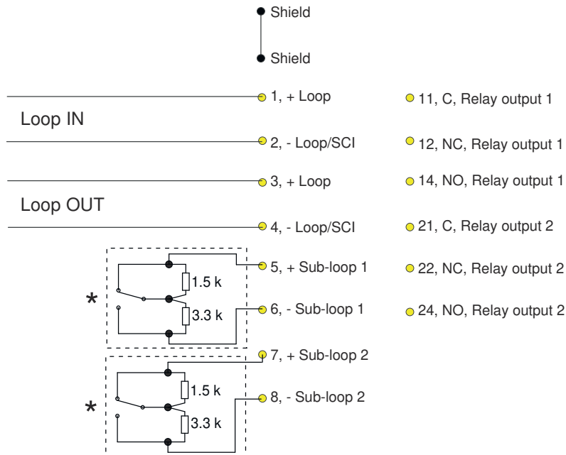
Figure 2. Terminals J101, J102 and J103
