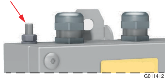
Figure 4. The M6 external earth connection
